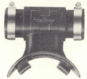
Cat. No. 1621 SCUBA NON-RETURN VALVE Includes: Cat. No. 1621-01 Mouthpiece Cat. No. 1621-02 Nylon inserts (two) Cat. No. 1621-03 Non-return rubber valves (two) Cat. No. 1621-04 Hose clamps (two) Cat. No. 1621-05 Baffle Retail $4.95
