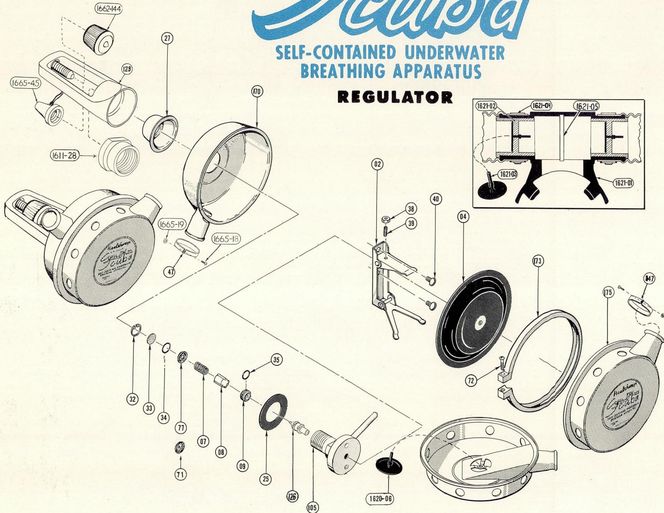
CATALOG NO. 1611—SCUBA REGULATOR "MODEL 1962"
