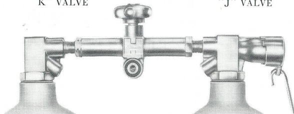
TWIN "J" VALVE
