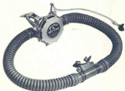
D1C "SCUBA 1 STAGE" OVERPRESSURE BREATHING BRIGHTCHROME HOUSING
