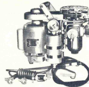
2500 PSI 0.6 CFM Free Air
