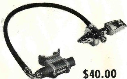
D2A SCUBA "PRO" DEMAND STAGE IN MOUTHPIECE
