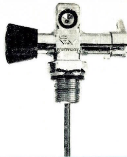
"SJ" CONSTANT RESERVE VALVE
